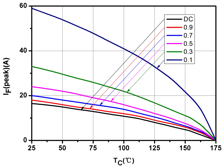
Fig.7-Current Derating
